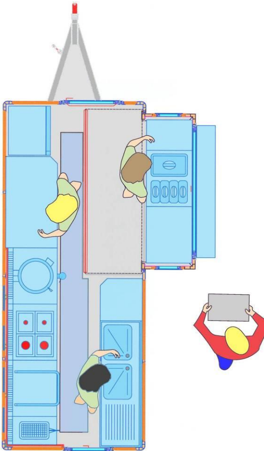
View/plan view of the overall unit in operating conditions
