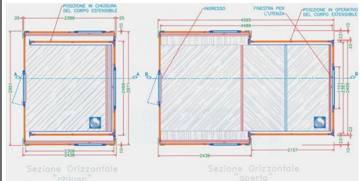
Sectional drawing horizontal "closed"
