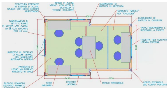
Section in the plant in the operating position
