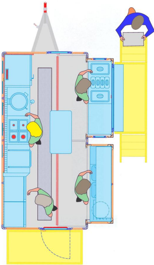
View/plan view of the unit in operating conditions
